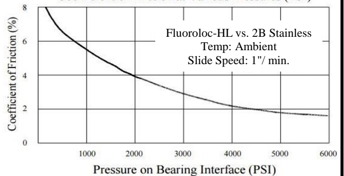
Coefficient of Friction at Various Pressures (PSI)
