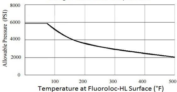
Design Pressure vs. Temperature
